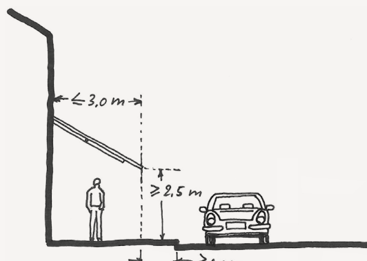
Figure 2 : Saillies mobiles
